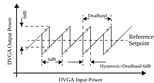
Figure 31 AGC Setup.
