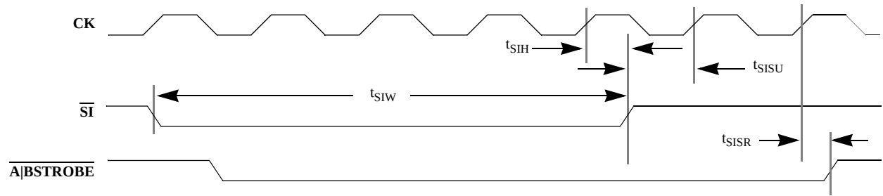
Figure 6 CLC5902 Synchronization Input ( \overline{\text{SI}} ) Timing
