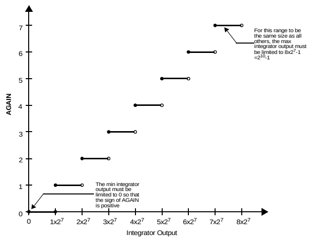
Figure 36 AGC integrator output limits
