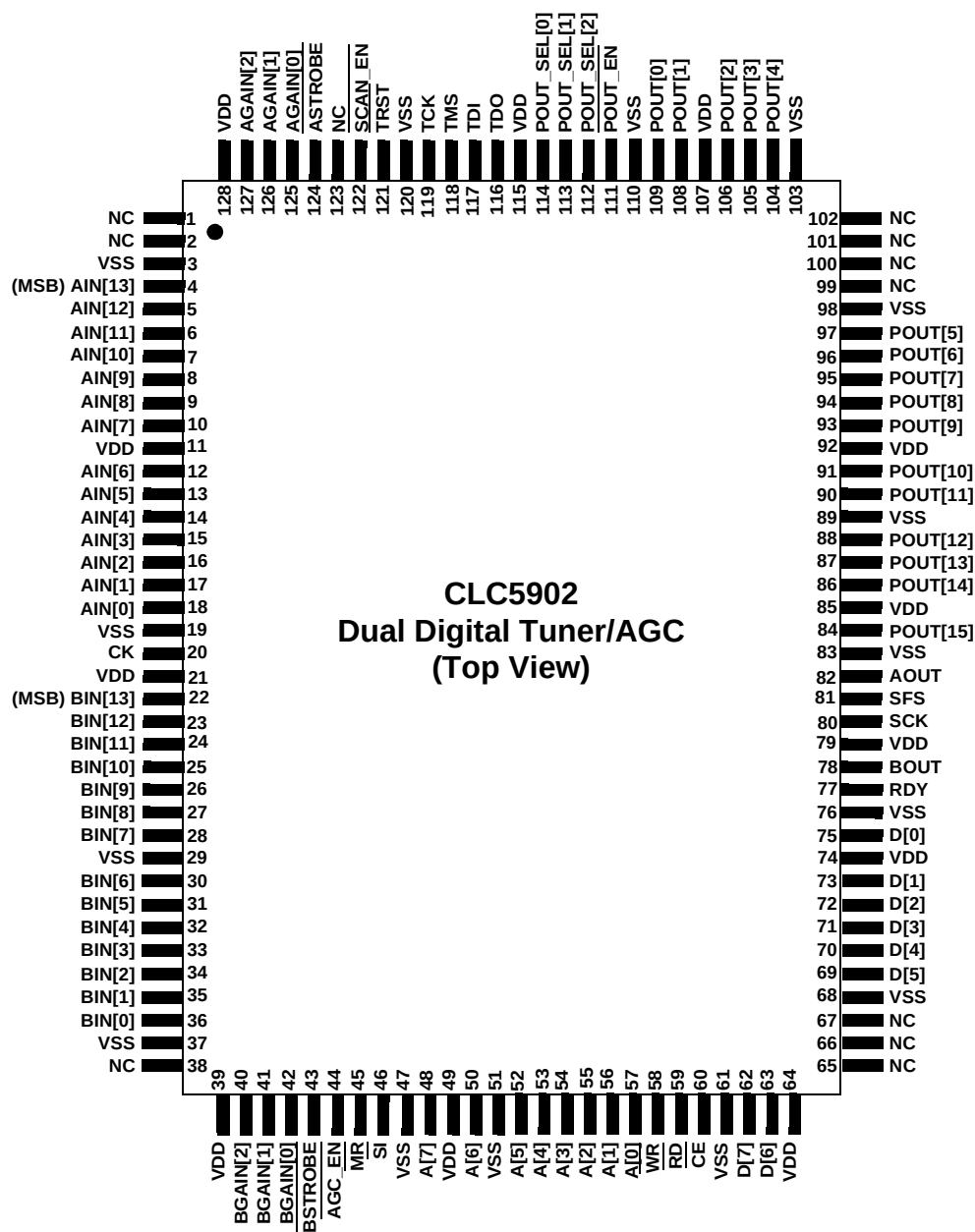
Figure 4 CLC5902 Pinout
